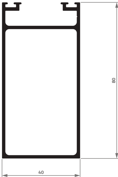
FC-012 1,200 Kg/m
