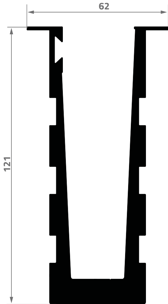
GR-U-02 4,883 Kg/m
