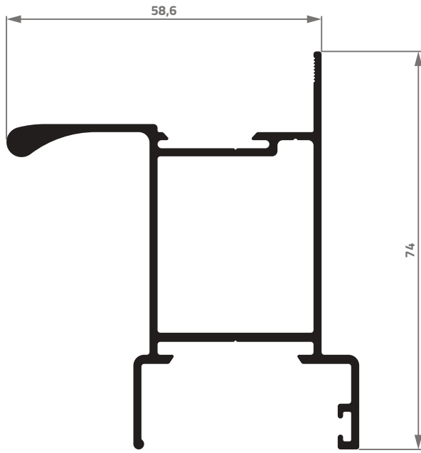
AG-020 1,116 Kg/m
