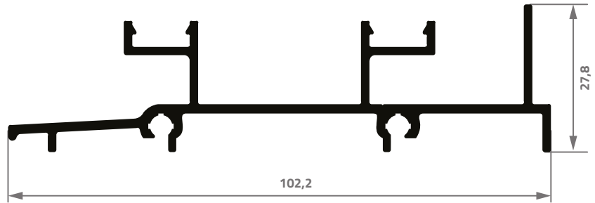
AG-125 1,008 Kg/m
