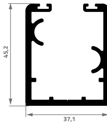
CEG-500 1,050 Kg/m
