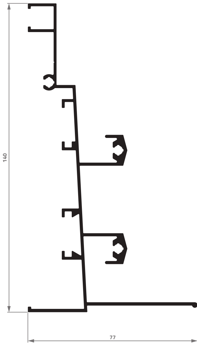
MN-030 1,643 Kg/m
