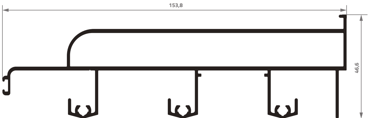
AG-034 2,149 Kg/m
