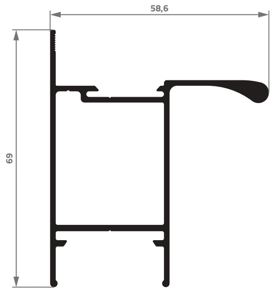
AG-017 1,009 Kg/m
