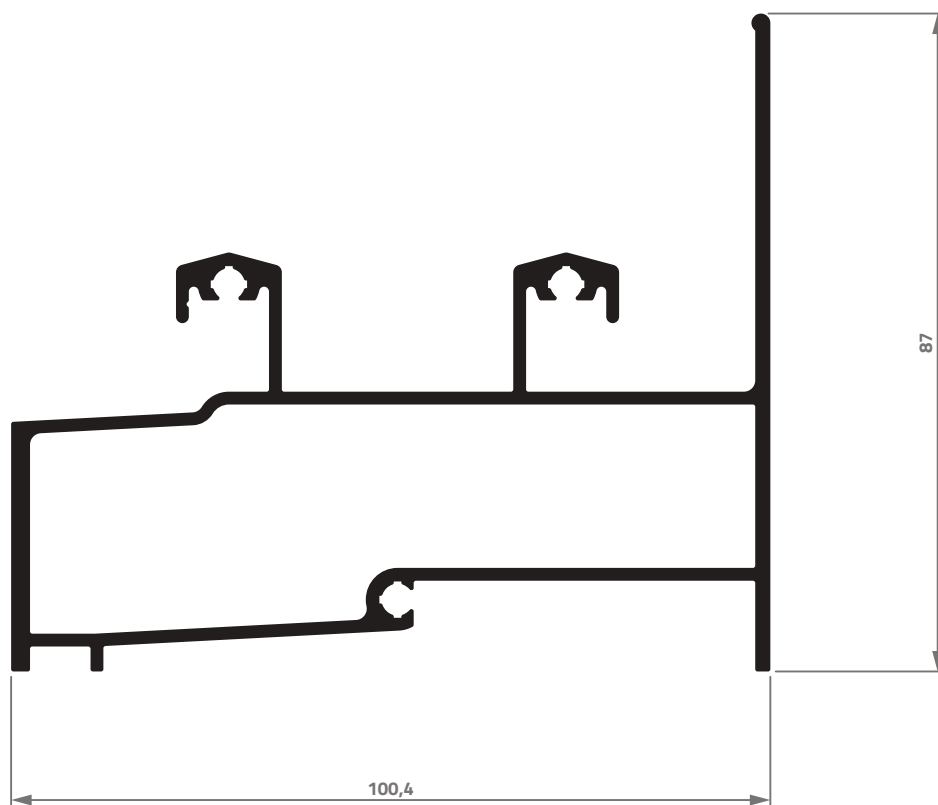
AG-005 2,103 Kg/m
