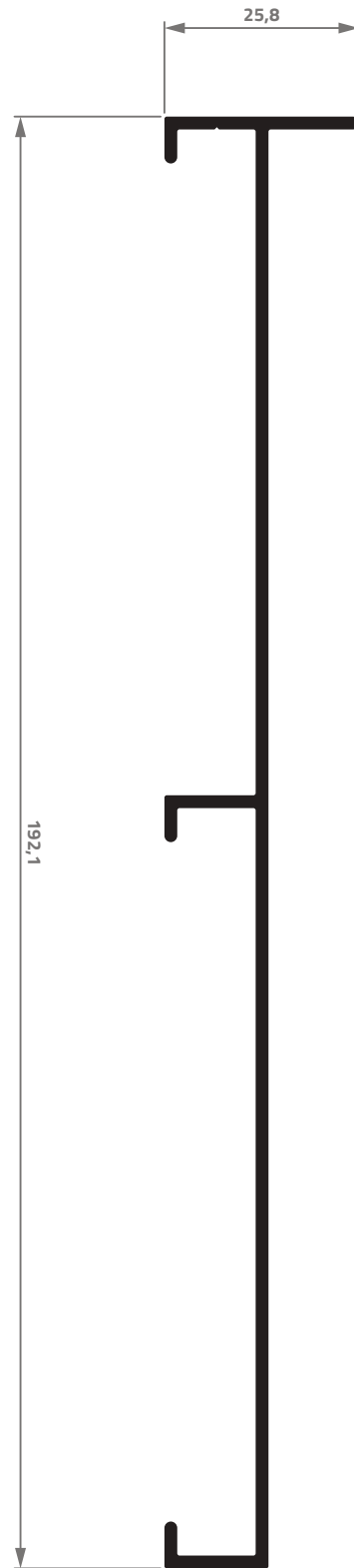
AG-072 1,166 Kg/m
